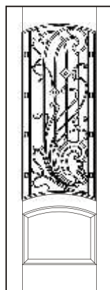
NHF 8832BVI & Grille 002 3'0" x 8'0" x 2 1/4"
