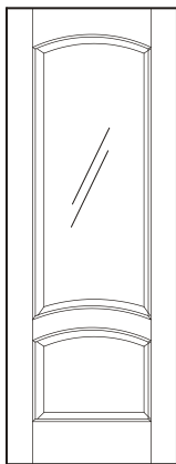
NHF 5761CIG & NHF 5761S 3'0" + 1'4" x 7'0" x 2 1/4" One Set is available with Frosted Glass.
