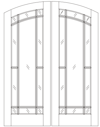
NHF 8804BVI Double Door 3'0" + 3'0" x 8'0" x 1 3/4"
